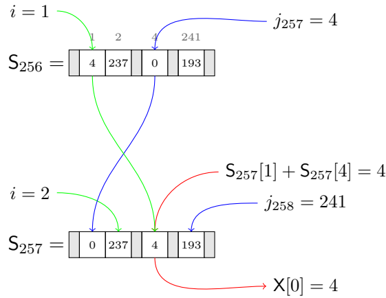
Figure 6.4: First key stream byte for K = 3, 255, 232, 251, 20, 158, 18, 173
